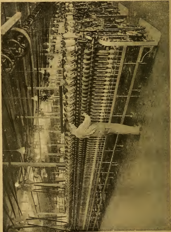
ENGLISH CAP SPINNING
